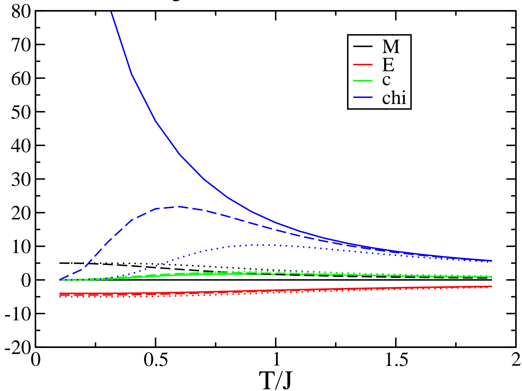
Ising 1D N=5 , J=1 , h=0.0/0.1/0.2
