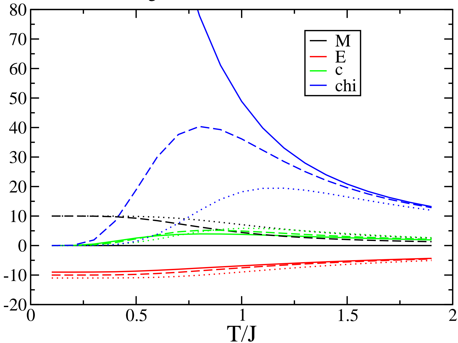
Ising1D N=10, J=1, h=0.0/0.1/0.2
